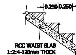
STAIR CASE DETAILS SCALE 1:25
