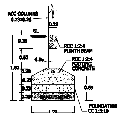
FOUNDATION DETAILS Scale 1:50
