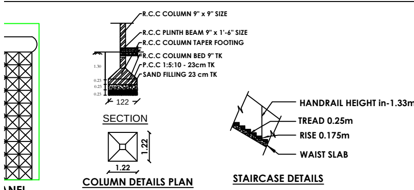
COLUMN DETAILS PLAN
