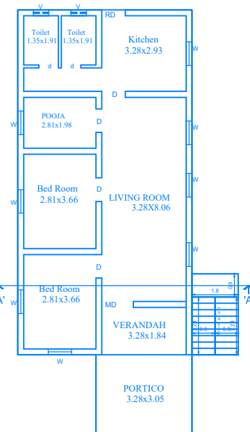
EXI.GROUND FLOOR PLAN
