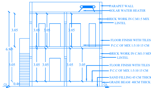
SECTION ON A-A1
