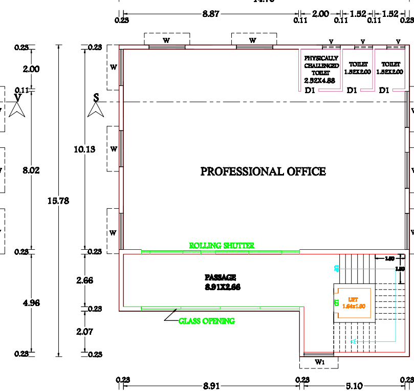
TYPICAL SECOND,THIED FLOOR PLAN
