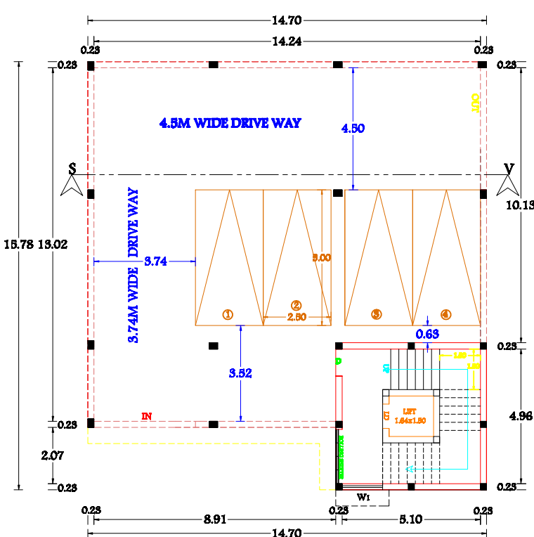
FLOOR PLAN
