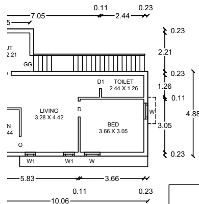
O-FIRST FLOOR PLAN
