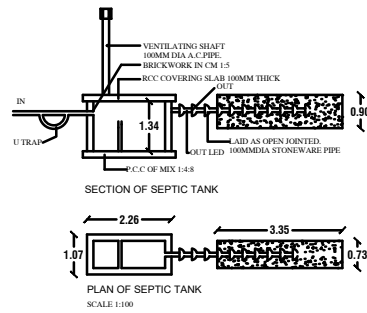
SECTION OF SEPTIC TANK SCALE 1:100
