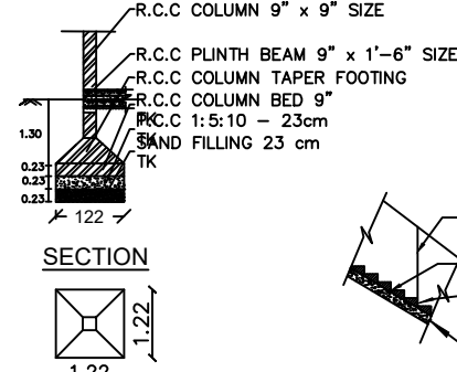
COLUMN DETAILS PLAN
