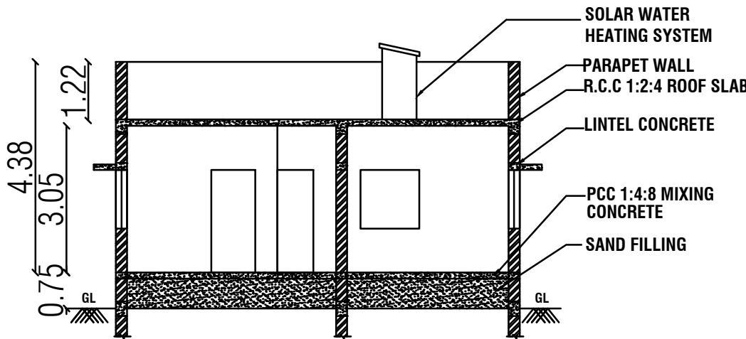
SECTION NO - "AB"
