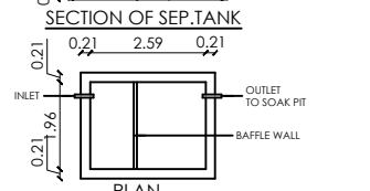
SEPTIC TANK
