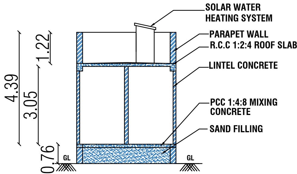
SECTION NO -"AB"
