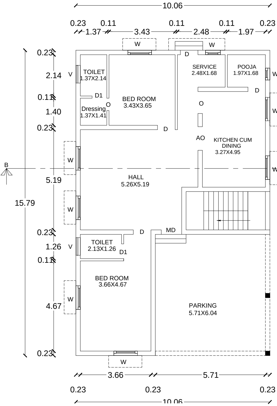
G.F. PLAN
