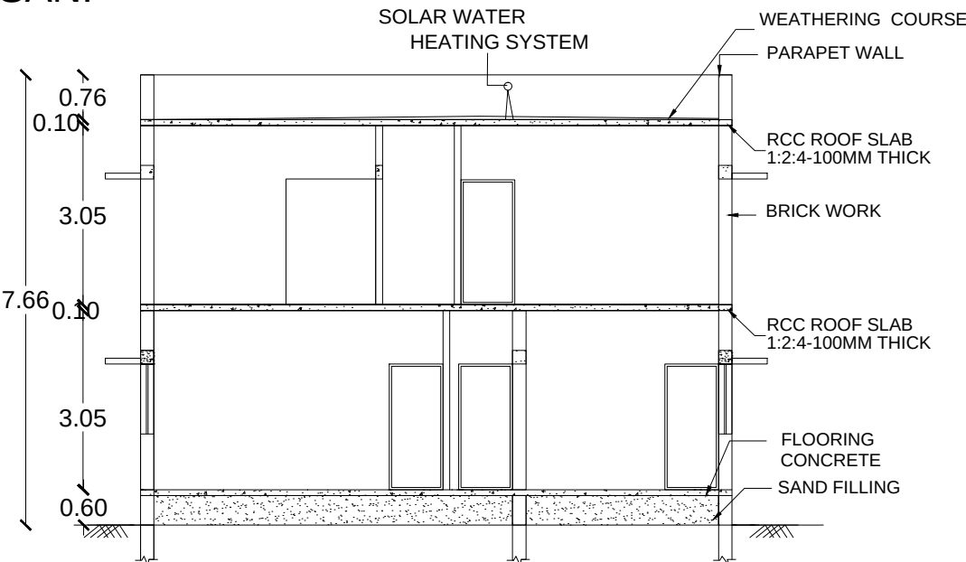
SECTION ON BR
