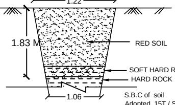
TRIAL PIT DETAILS NOT TO SCALE
