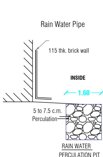
RAIN WATER PERCUSSION PIT
