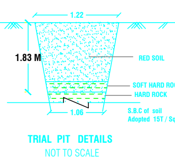
TRIAL PIT DETAILS
