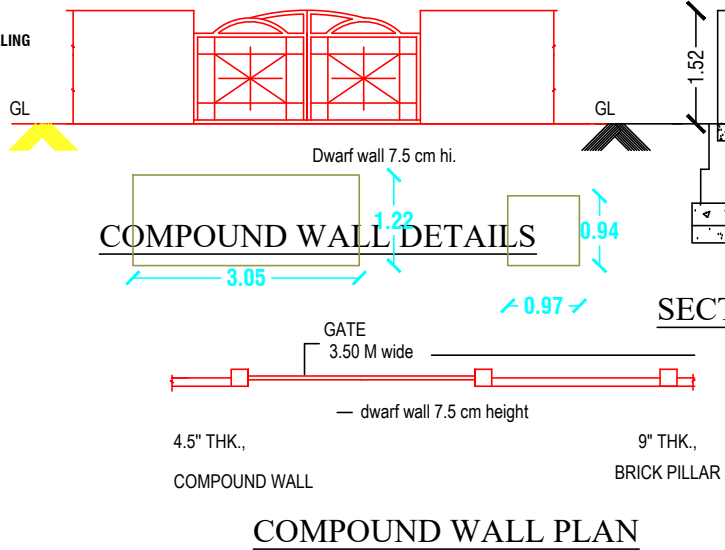
COMPOUND WALL PLAN
