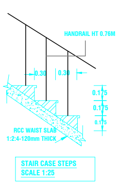
STAIR CASE STEPS
