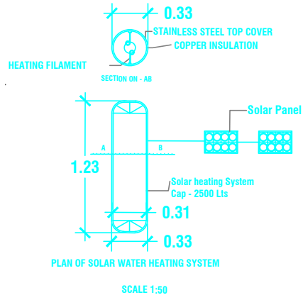
PLAN OF SOLAR WATER HEATING SYSTEM
