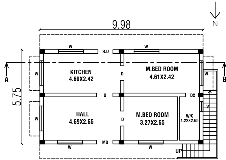
PRO.GROUND FLOOR PLAN
