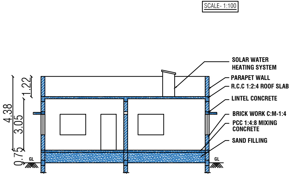
SECTION -"AB"
