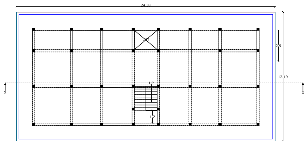
PROPOSED STILT FLOOR PLAN
