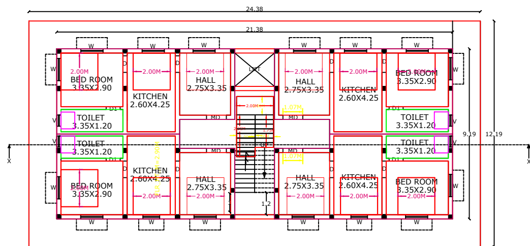
PROPOSED SECOND FLOOR PLAN
