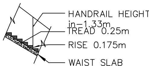
STAIRCASE DETAILS
