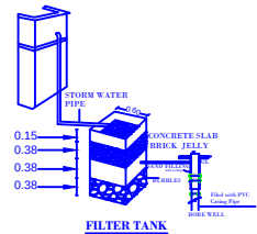
FILTER TANK
