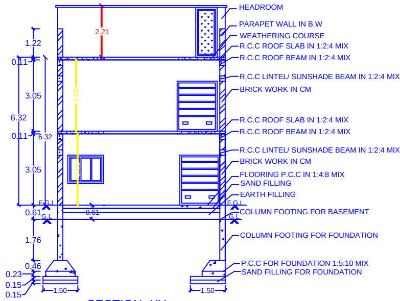
SECTION -XY
