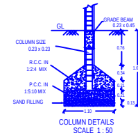
COLUMN DETAILS
