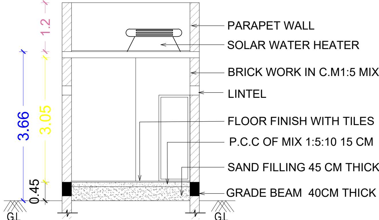
SECTION-AA
