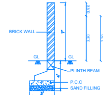
COMPOUND WALL DETAIL
