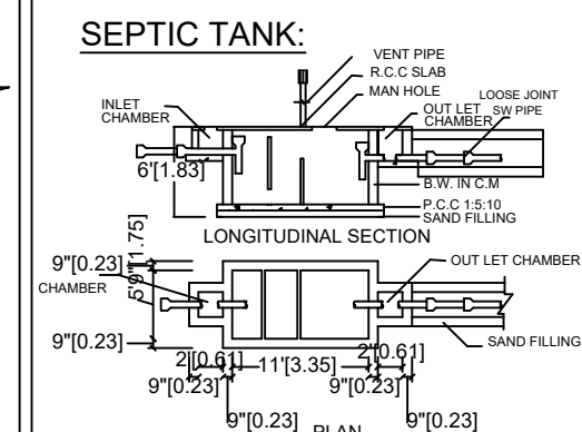
SEPTIC TANK:
