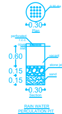
RAIN WATER PERCOLATION PIT
