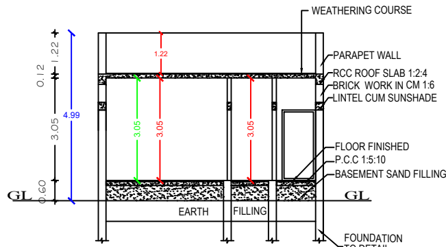
SECTION "J-J"
