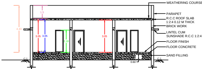
SECTION "N-R"
