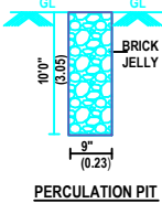
PERCOLATION PIT
