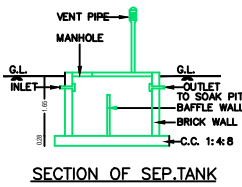
SECTION OF SEP.TANK
