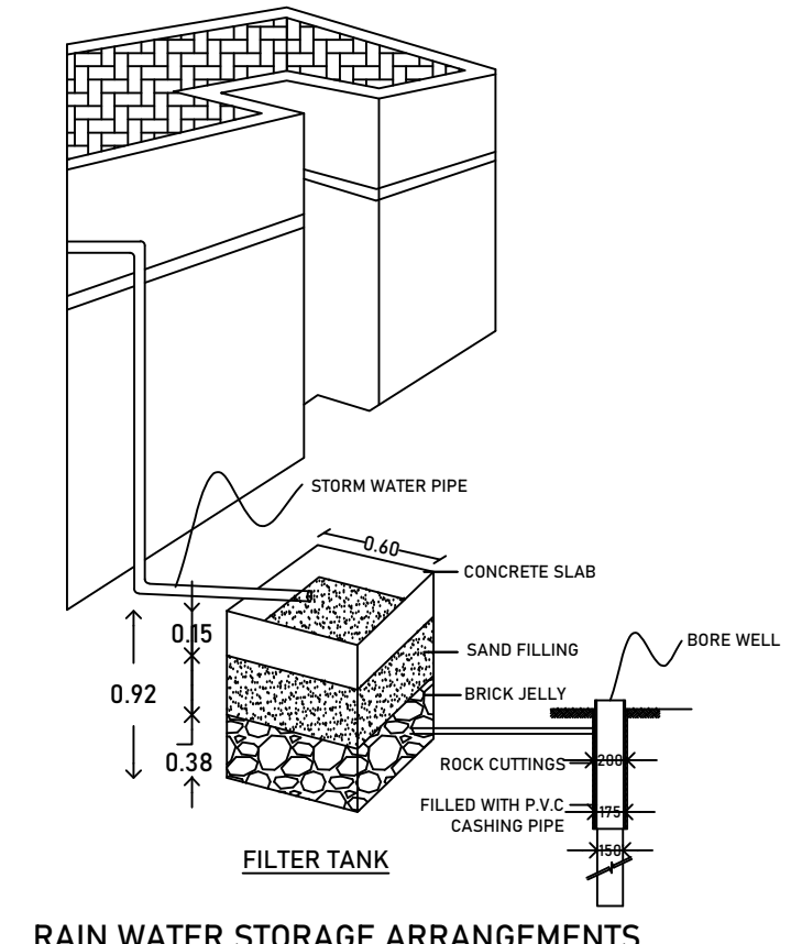
RAIN WATER STORAGE ARRANGEMENTS
