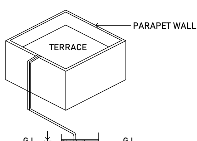
COLLECTION SUMP FOR HARVESTING FOR TERRACE
