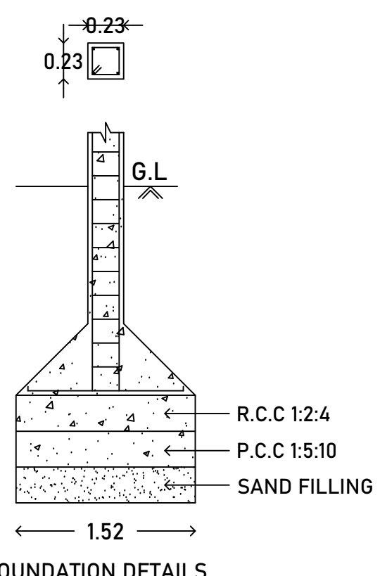
FOUNDATION DETAILS
