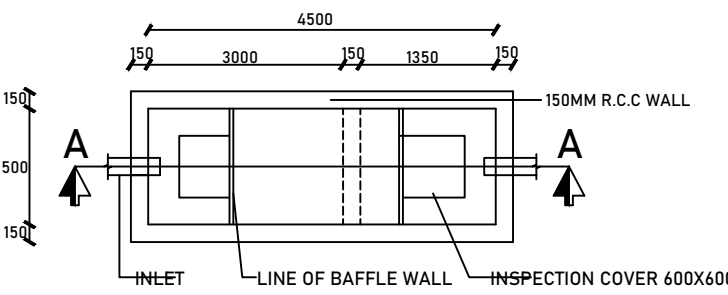
PLAN OF SEPTIC TANK SIZE 4.5M X 1.5M X 2.0M [ 400 LITERS / DAY ]
