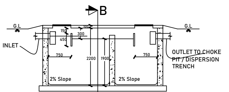
SECTIONAL ELEVATION - AA
