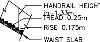
STAIRCASE DETAILS
