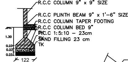
SECTION
