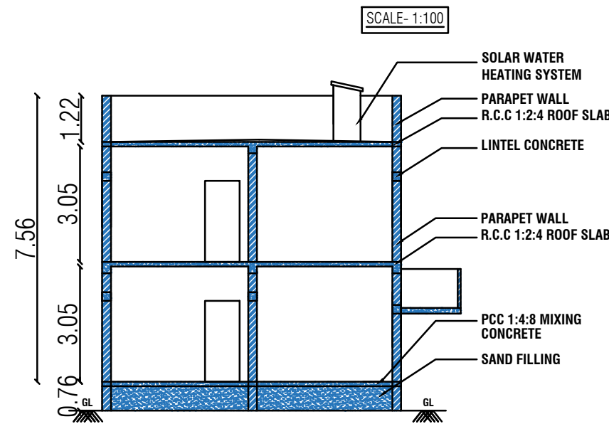
SECTION NO - "AB"
