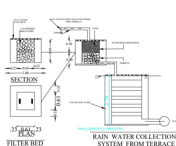
PLAN FILTER BED
