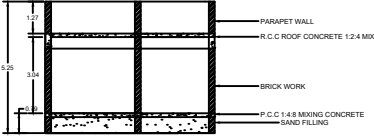
CROSS SECTION
