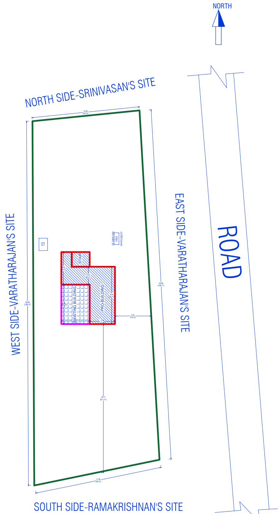
SITE PLAN
