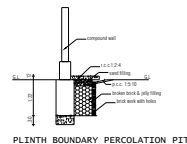
Proposed Details:
