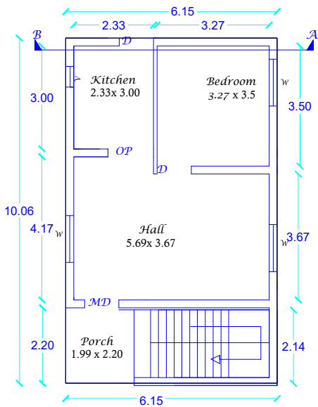
ADD. GROUND FLOOR PLAN
