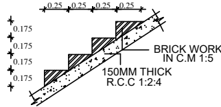
STAIRCASE DETAILS NOT TO SCALE
