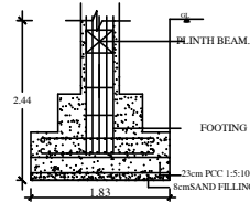
COLUMN FOUNDATION DETAILS NOT TO SCALE
