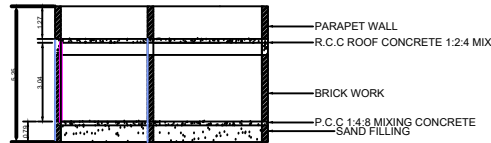
CROSS SECTION
