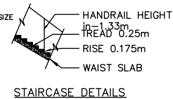
STAIRCASE DETAILS
