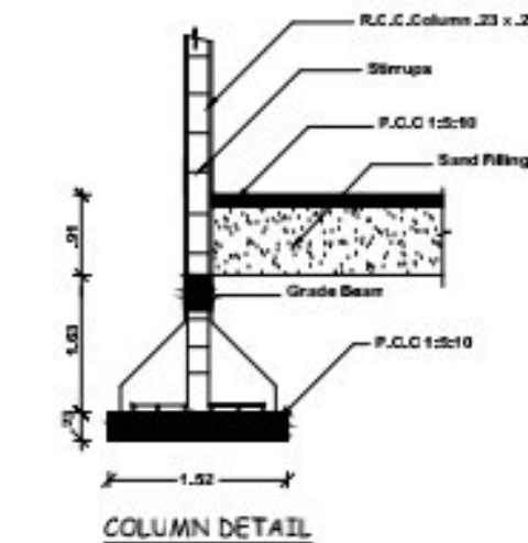
COLUMN DETAIL
