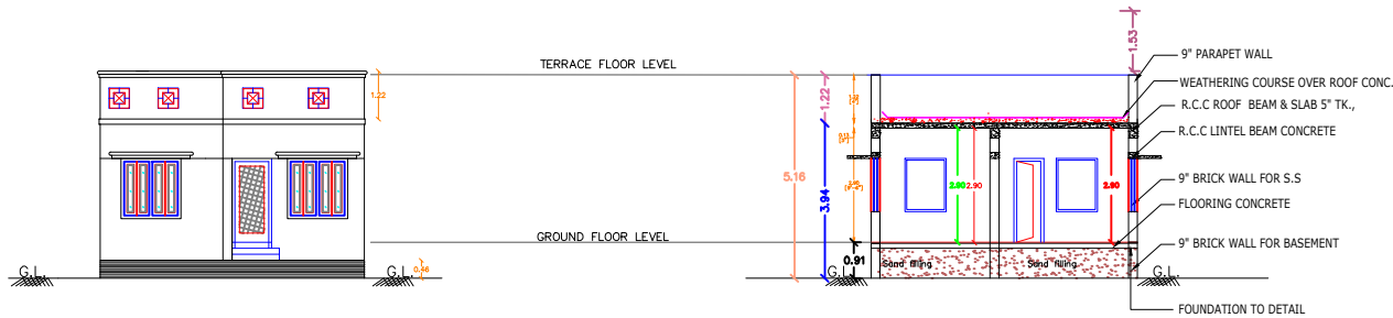
FRONT ELEVATION
