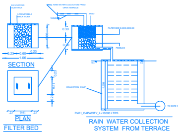
RAIN WATER COLLECTION SYSTEM FROM TERRACE
