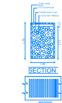
RAIN WATER HARVESTING PERCOLATION BED
