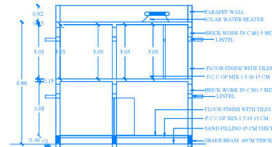
SECTION ON A-A1
