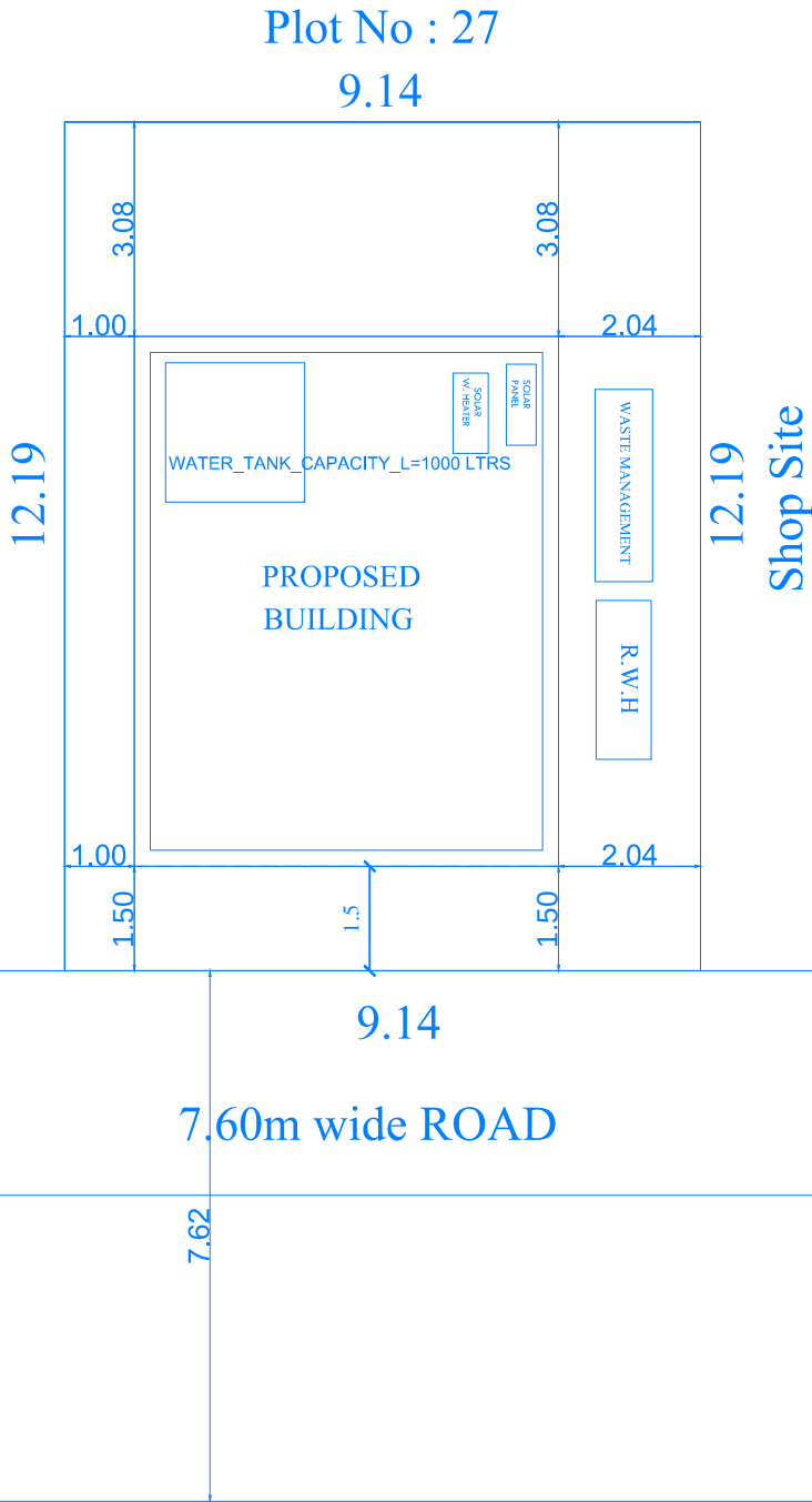
SITE PLAN
