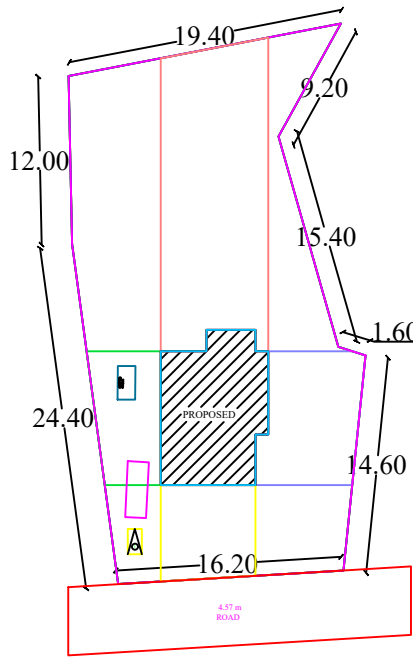
SITE PLAN
