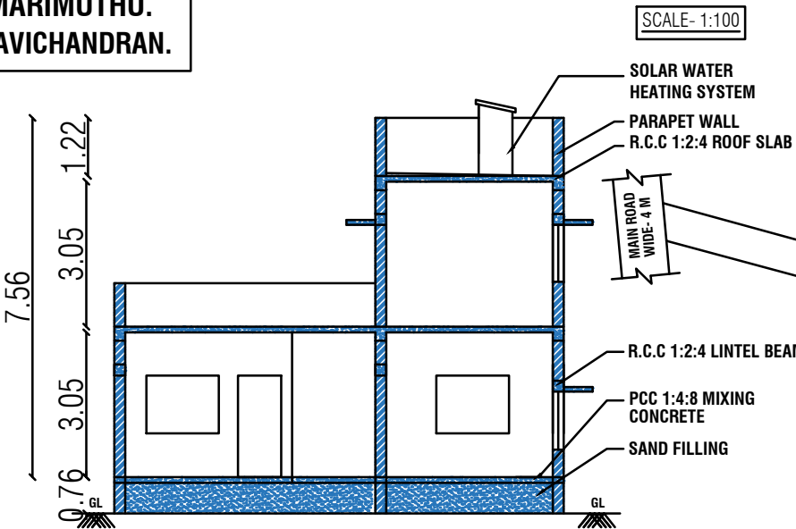
SECTION NO - "AB"
