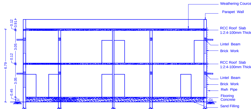
SECTION X-Y
