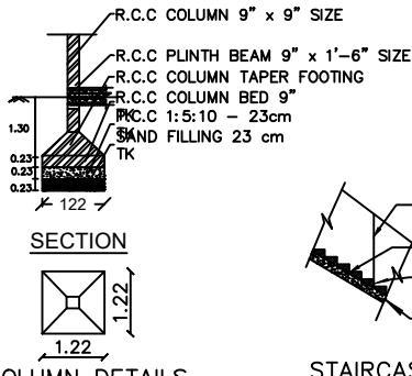
COLUMN DETAILS
