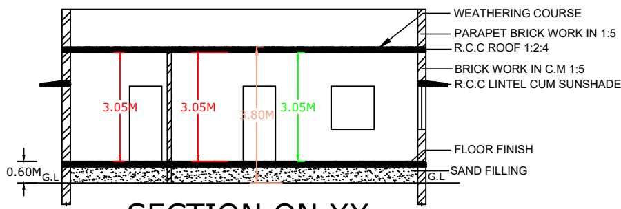
SECTION ON XX
