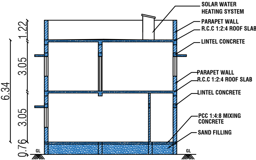
SECTION NO -"AB"
