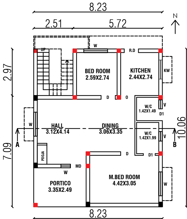
EXI.GROUND FLOOR PLAN
