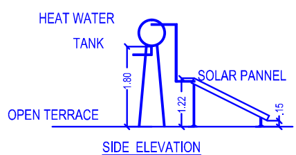
HEAT WATER TANK SIDE ELEVATION
