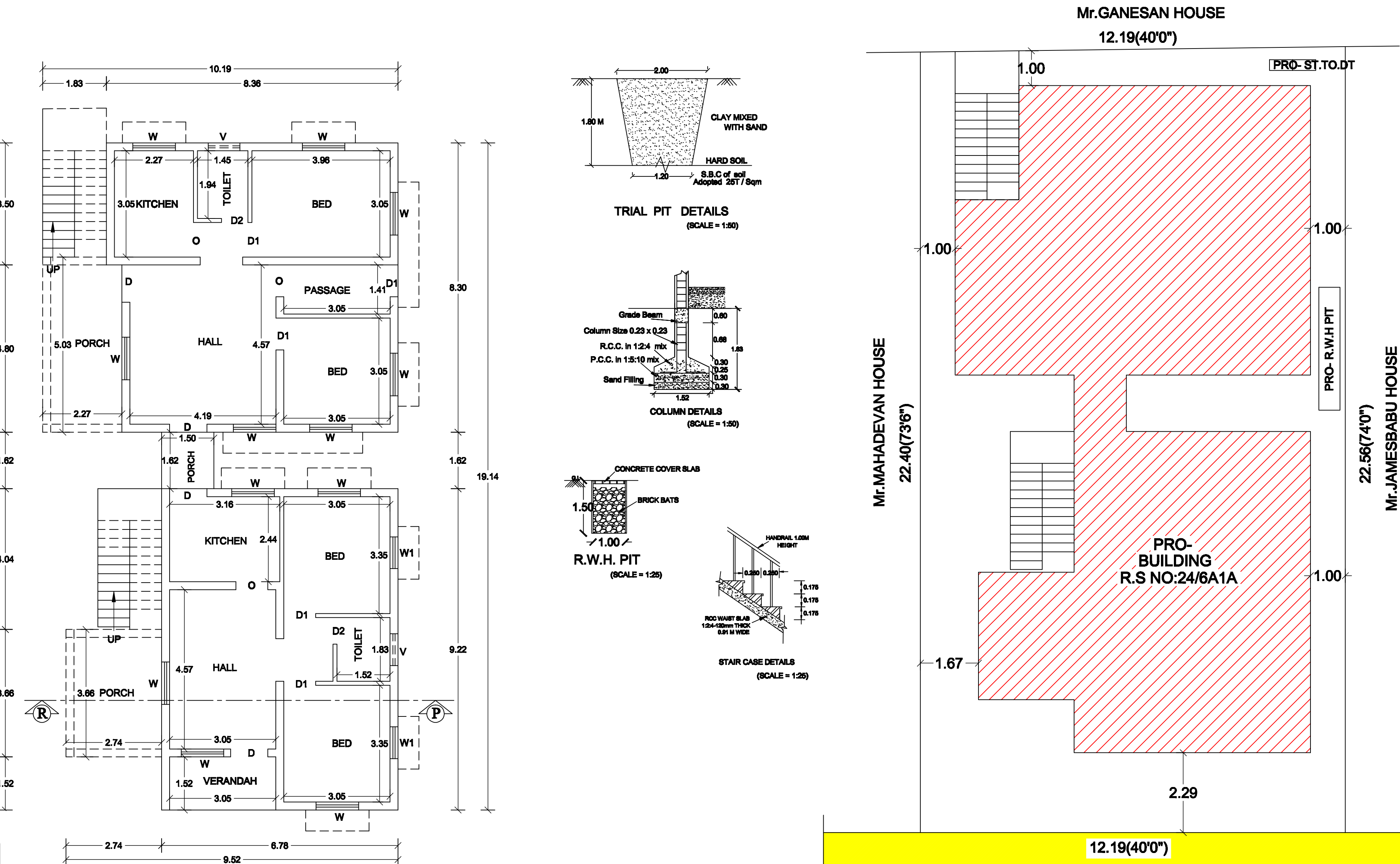
PRO- GROUND FLOOR PLAN
