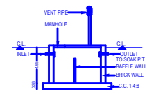
SECTION OF SEPT.TANK
