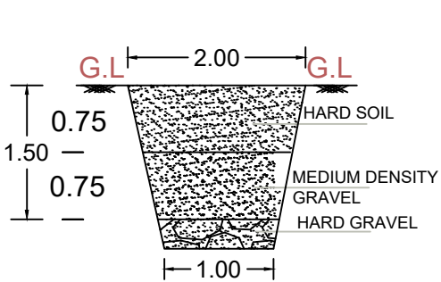
TRIAL PIT
