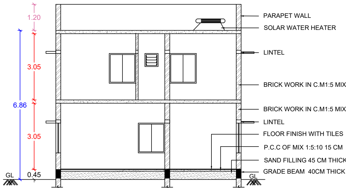
SECTION- AA1
