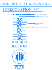
RAIN WATER HARVESTING SYSTEM
