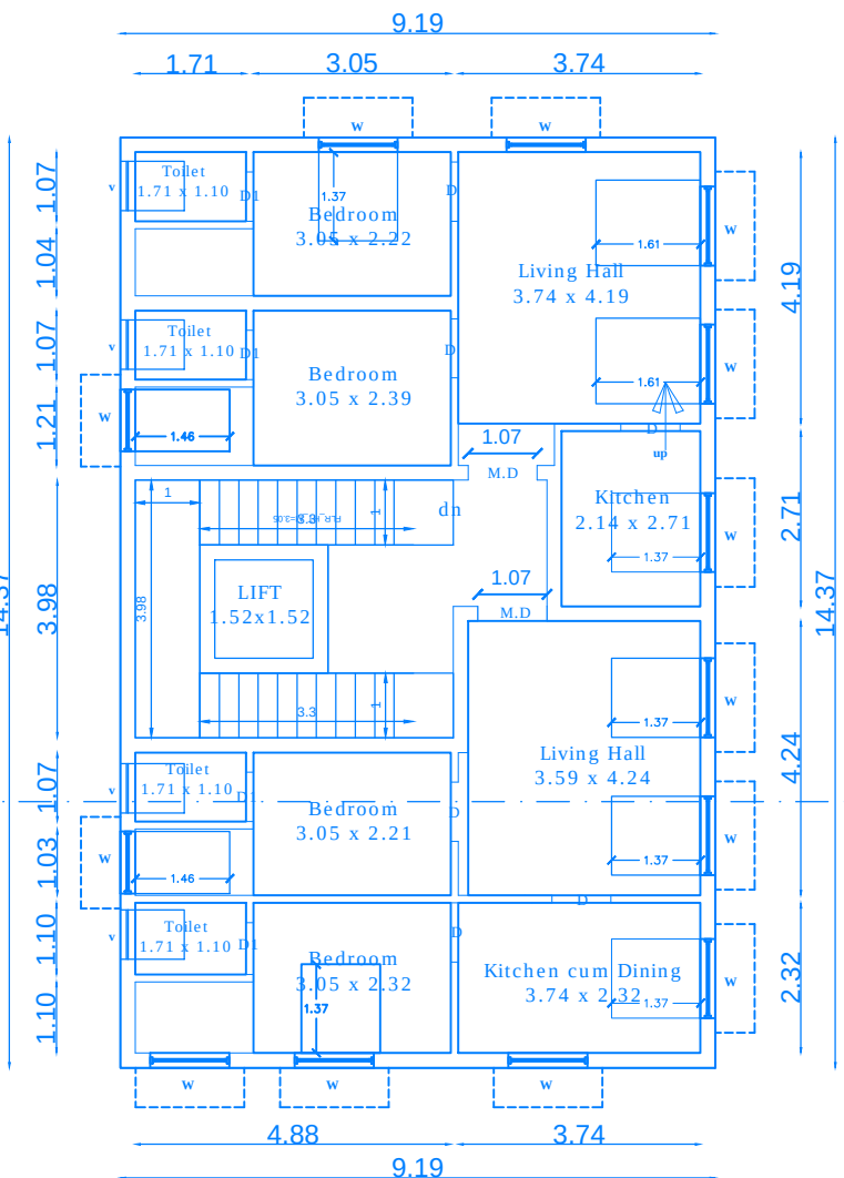
TYPICAL FIRST, SECOND & THIRD FLOOR PLAN
